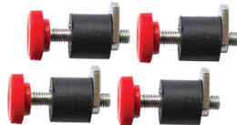
Motor Isolation Mounts 4-Pack HEPMIMT1004
